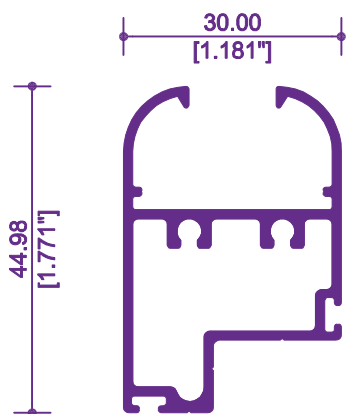
3503 / 12274 MARCO COLONIAL
