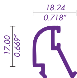
4593 / 62030 JUNQUILLO 24mm.
