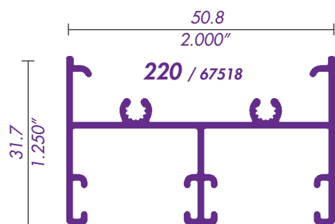
JAMBA CONTRAMARCO W
