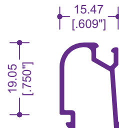
5085 / 12576 JUNQUILLO COLONIAL
