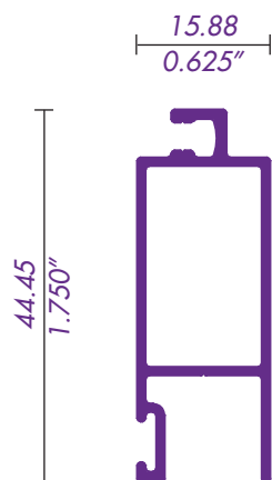
209 / 66534 MOSQUITERO VERTICAL
