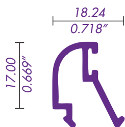
4593 / 62030 JUNQUILLO 24mm.
